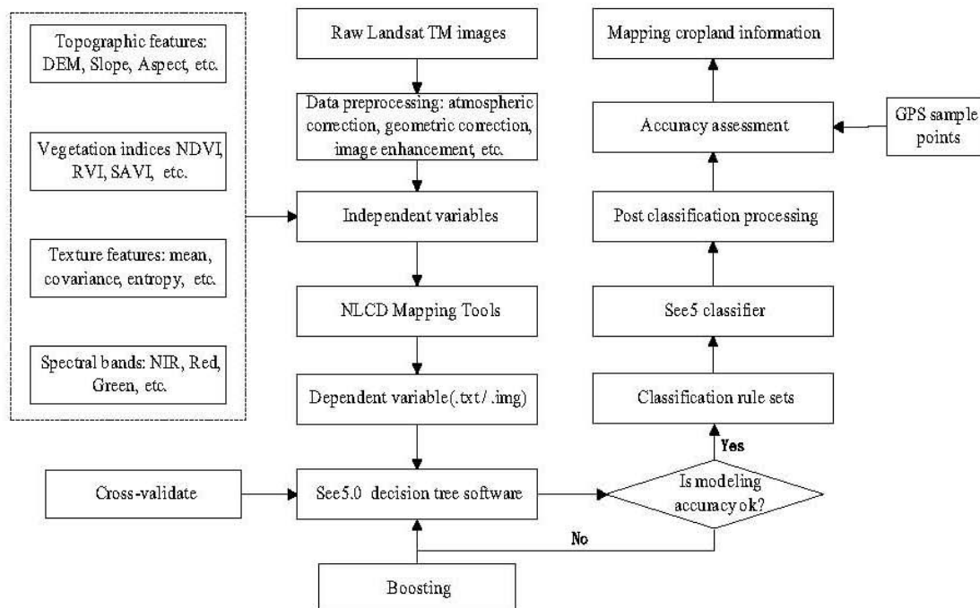
Fig. 2. Overall flow chart for identifying croplands integrating NLCD mapping tools and See5 decision-tree software
